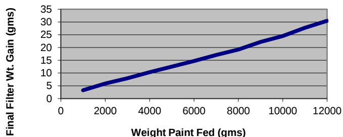
Removal Efficiency
