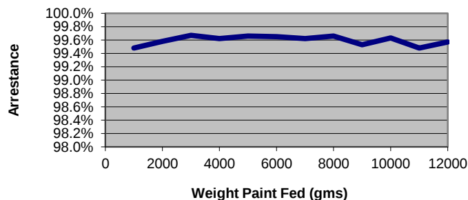
Removal Efficiency
