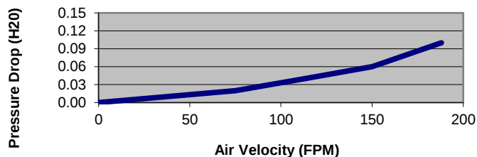
Pressure Drop
